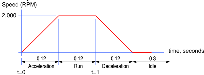
Figure 8 – Move profile
